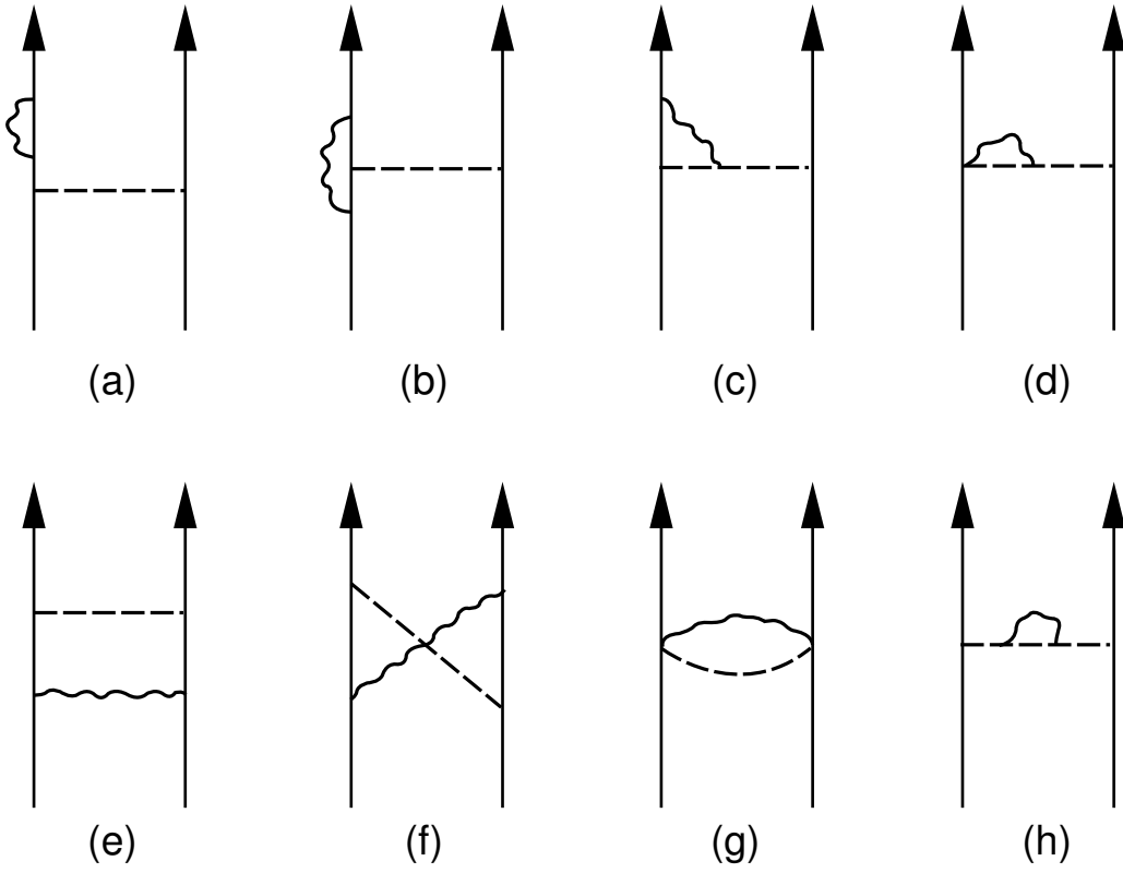
FIG. 1. Electromagnetic loops contributing to isospin violation in the OPE nuclear force in leading order. Solid lines are nucleons, dashed lines are pions, and wavy lines are photons.
